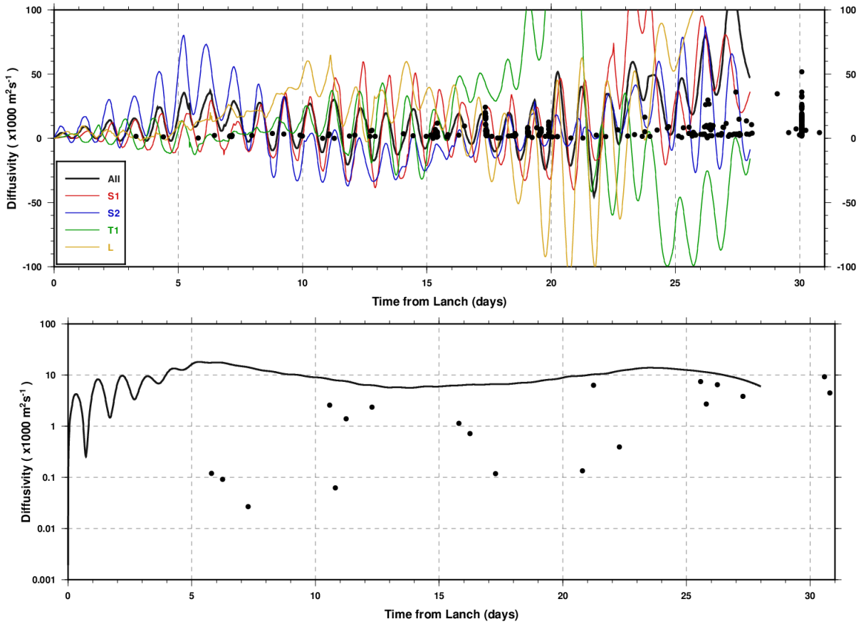
Figure 13: The top panel is the horizontal diffusivity K , in 10^3 \text{ m}^2/\text{s} , as a function of time after deployment in days for the primary drifter clusters. Note that the smallest and largest values fall outside the axis limits here. The minimum and maximum values of K are from cluster L and are -110 \times 10^3 \text{ m}^2/\text{s} and 360 \times 10^3 \text{ m}^2/\text{s} , respectively. The dots show the horizontal diffusivity calculated by Taylor’s method as described in the text. The solid line in the bottom panel is a spline-smoothed version of the ALL curve from the top figure on a log scale. The dots are an average of all of the Taylor-based estimates for each of the temporal midpoints of the 31-day data segments.
