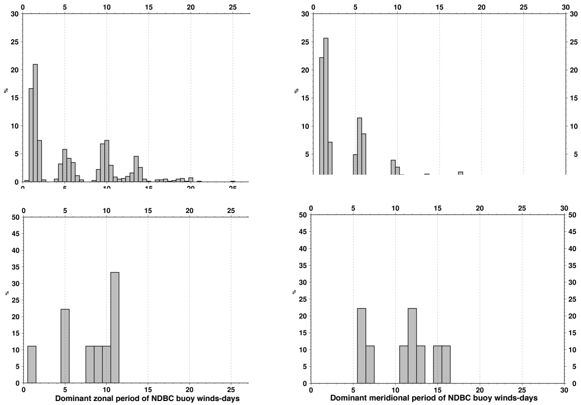
Figure 7: The top panels are the histograms of the dominant period, in days, of the (left) u and (right) v velocity components for all estimates calculated from the GLAD drifters. The vertical axis is the percentage of samples in each bin. The bottom panels are the histograms of the 10 m (left) zonal and (right) meridional wind velocity components dominant period calculated for 8 NDBC wind data sets for the same time period.
