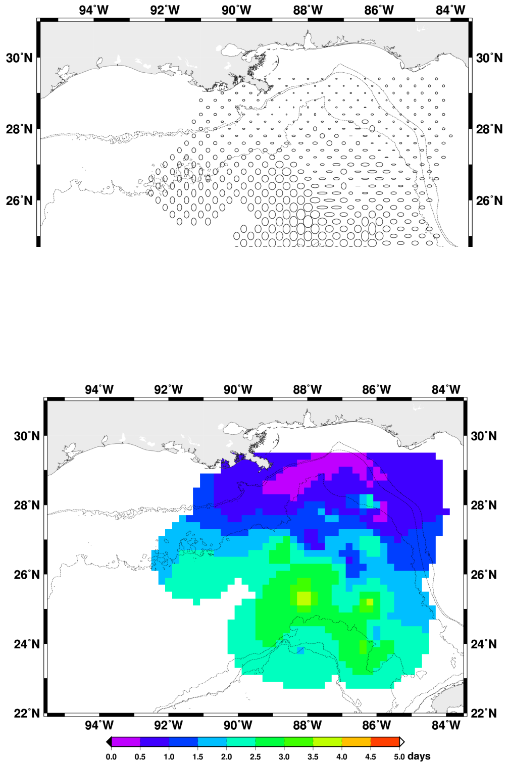
Figure 11: The top panel is a map of the ellipses of the integral time scale, in days, for the surface velocity field in the northern Gulf of Mexico. The bottom panel is the amplitude of the integral time scales, I = \sqrt{T_u^2 + T_v^2} . Units are days.
