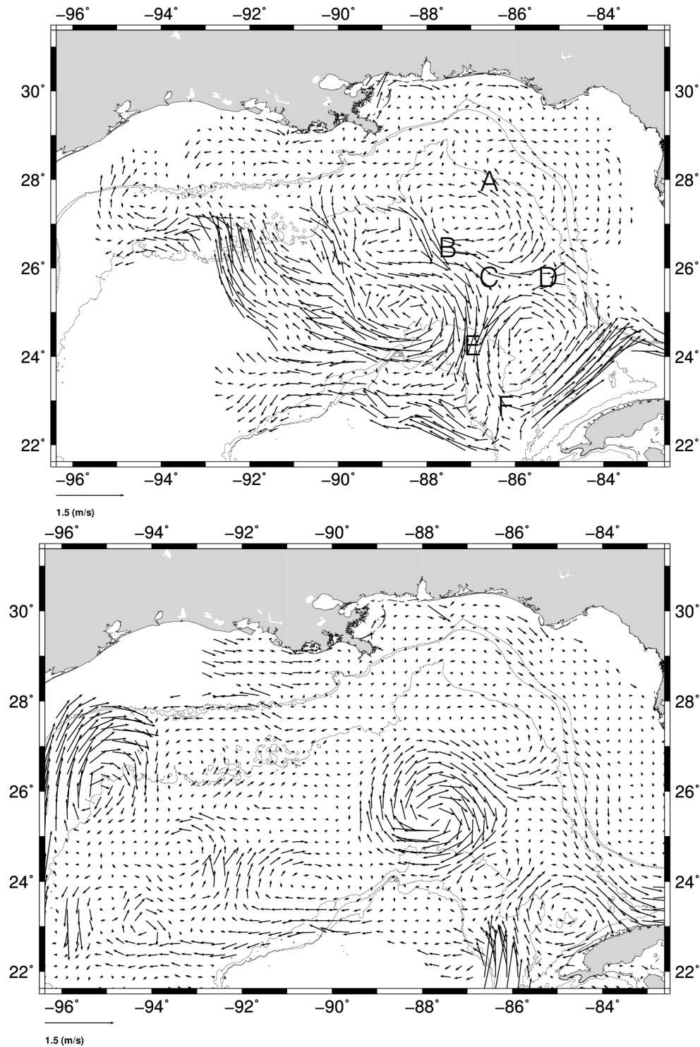
Figure 3: (Top) Average velocity from the same GLAD drifter data used in Fig. 2, but based on a new localized, minimum-variance, adaptive coordinate system blending technique (see text). The symbols A, B, C, D, E, and F indicate regions of flow bifurcations. (Bottom) Climatological average velocity from the Atlantic Oceanographic and Meteorological Laboratory (AOML) archived near-surface drifters for the summer months July, August, and September, and for the years 1996-2013. The 200 m, 300m, and 2000 m isobath contours are also plotted.
