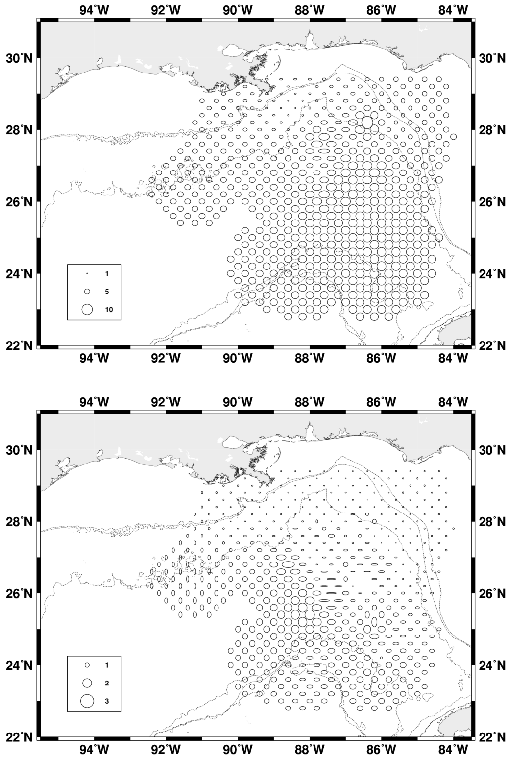
Figure 9: The top panel is a plot of the dominant period ellipses, in units of days, for both the u and v velocity components. The bottom panel is a plot of the dominant e-folding scale ellipses, in units of days, for both the u and v velocity components.
