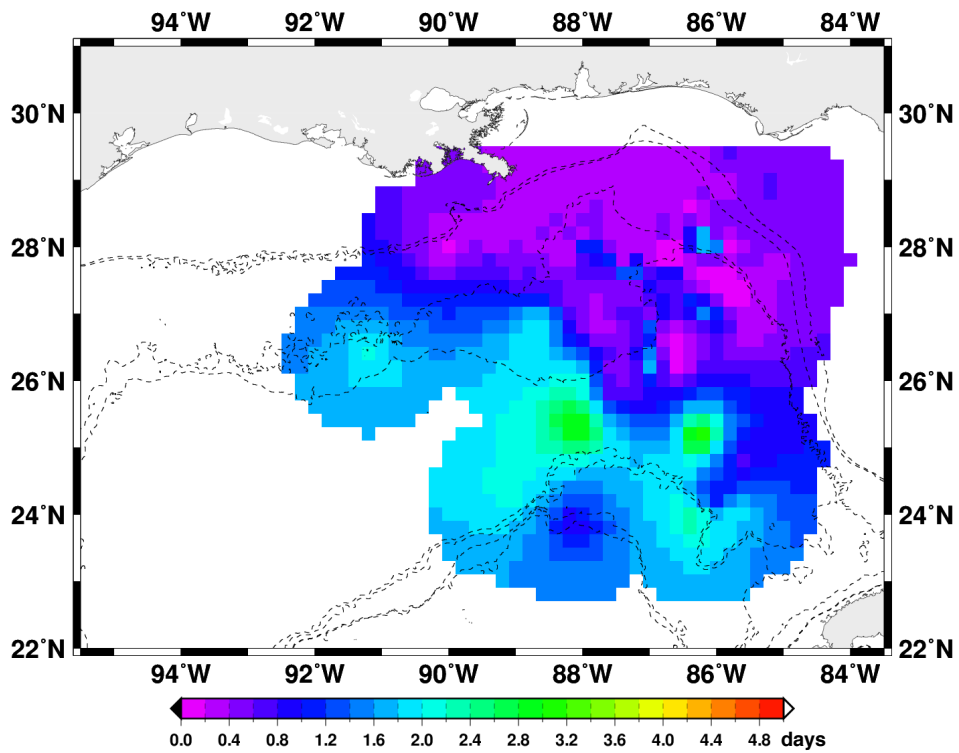
Figure 10: Maps of the integral time scale, in days, of the (top) u and (bottom) v velocity components.
