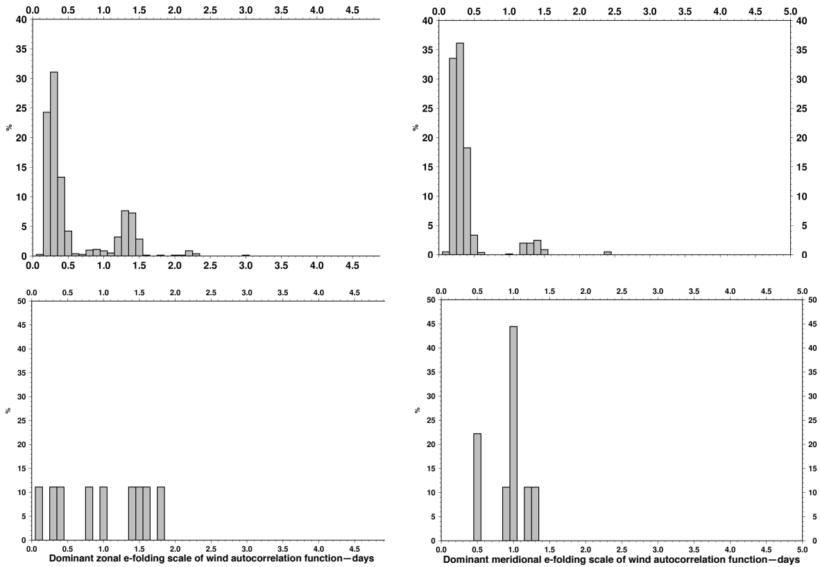
Figure 8: The top panels are the histograms of the dominant e-folding scales, in days, of the (left) u and (right) v velocity component for all estimates calculated from the GLAD drifters. The bottom panels are the histograms of the 10 m (left) zonal and (right) meridional wind velocity components dominant e-folding scales, calculated for 8 NDBC wind data sets for the same time. The vertical axis is the percentage of samples in each bin.
